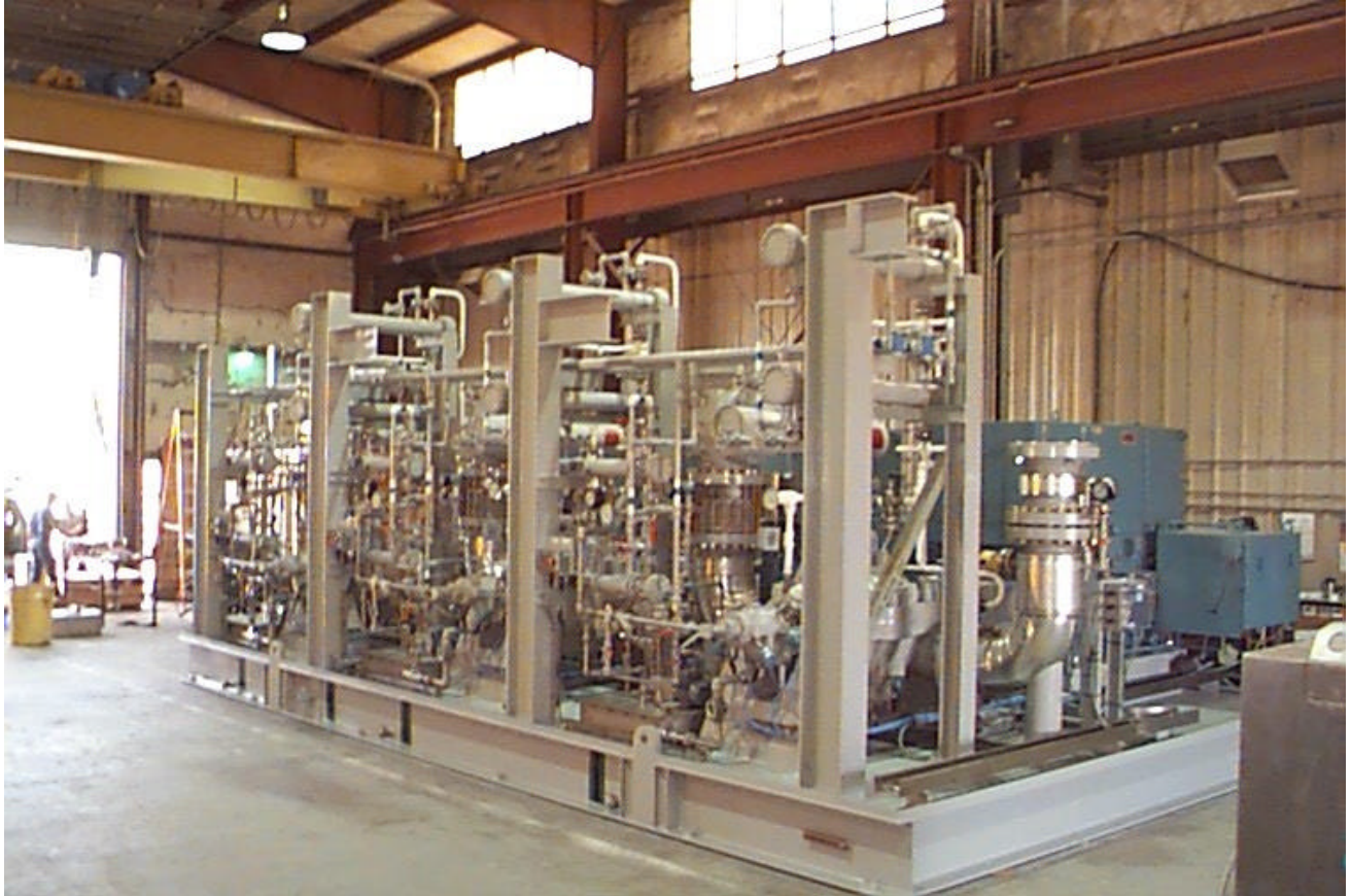
Crude Oil Shipping Pump Module installed on FPS in Offshore Brasil
