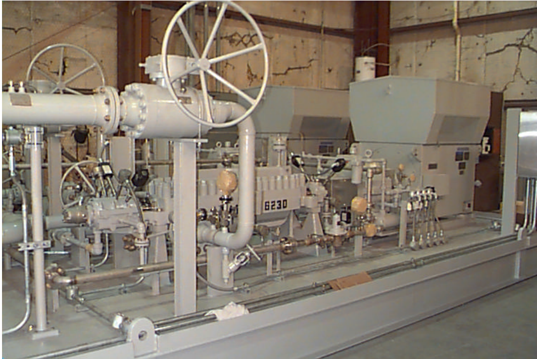
Water Injection Module – featuring IFS Remanufactured API-610 Pumps resulting in a very fast 15 week module shipment
