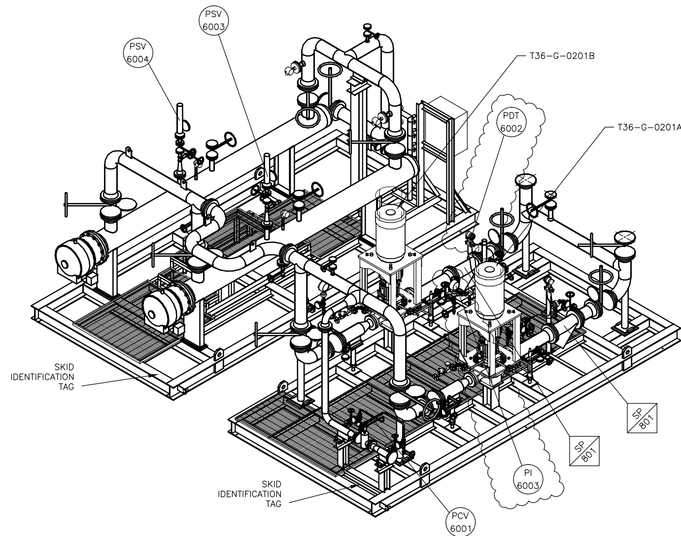
ISO VIEWS (FOR REFERENCE ONLY)
