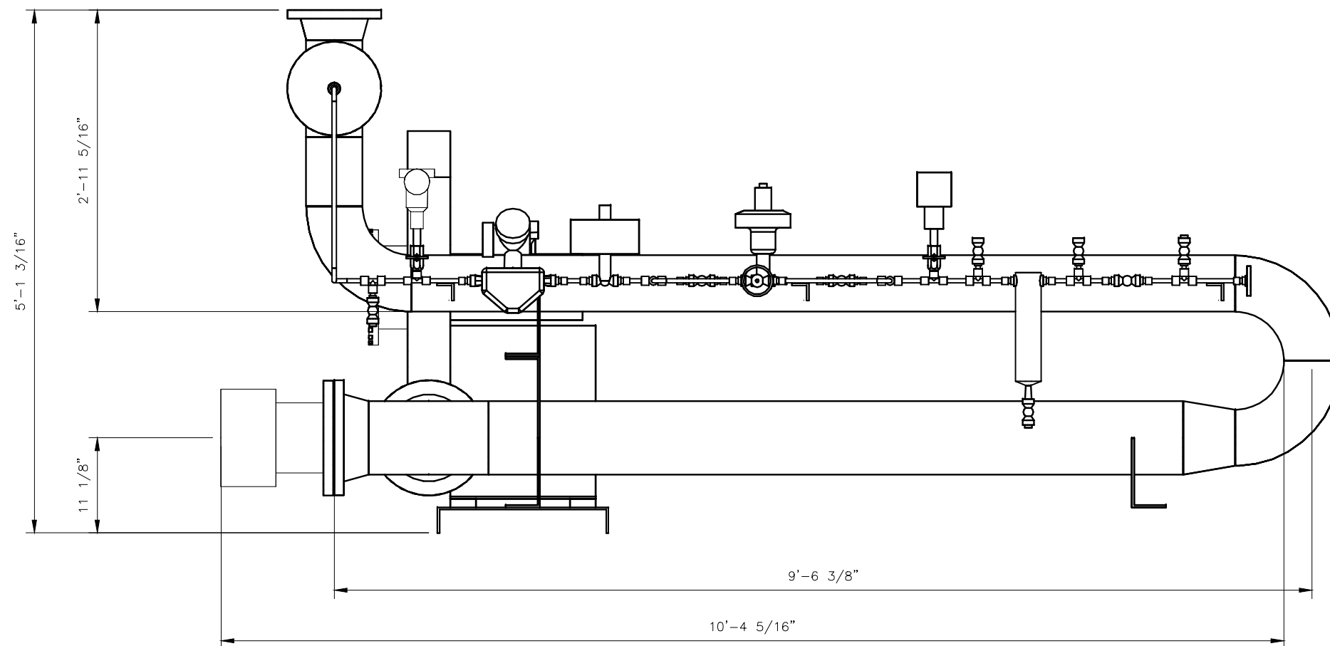
ELEVATION VIEW
