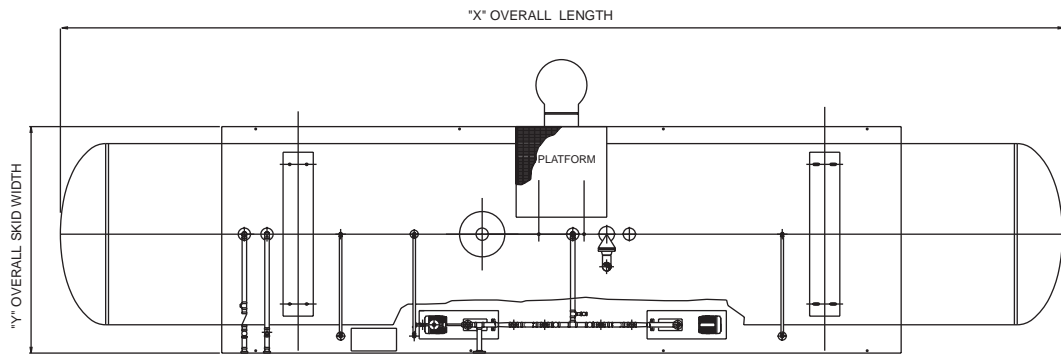
PLAN VIEW
